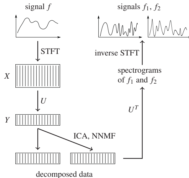
Fig. 5: Signal separation with dimensionality reduction.
