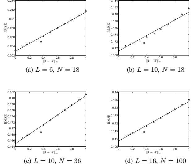
Fig. 2. RMSE for the Shepp-Logan phantom
