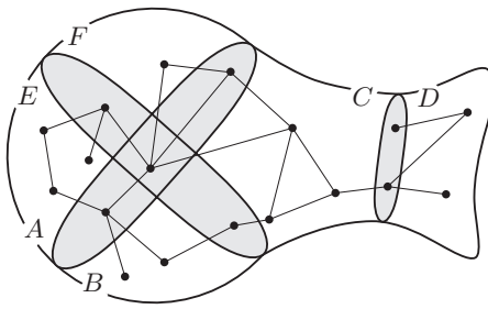
Figure 2: Separations as in Lemma 2.2
