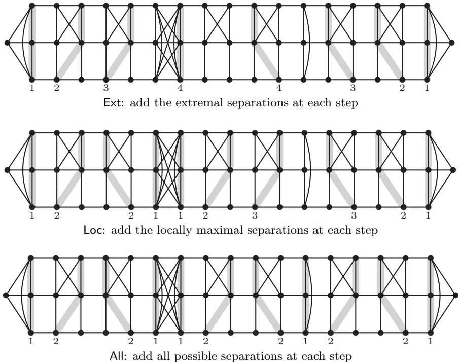
Figure 4: Three different nested separation systems distinguishing the 4-blocks profiles. It is not hard to show, and will follow from Lemma 4.1, that (S, \mathcal{P}) is a feasible task.
